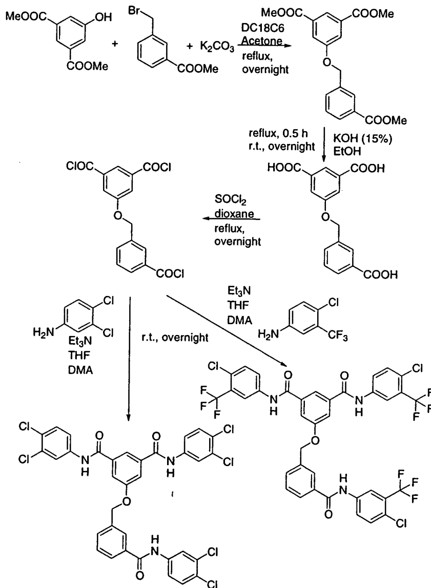
Scheme I-G
